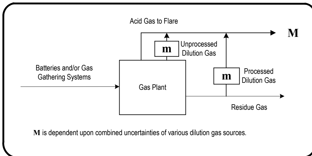
Figure 1.14 Dilution gas
