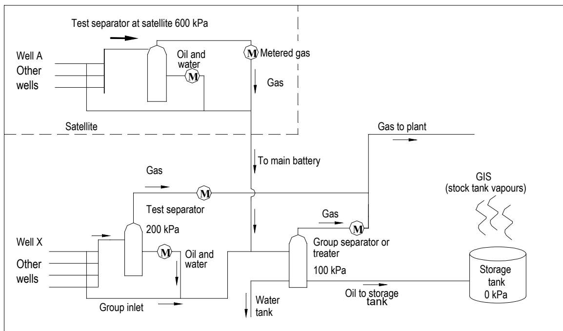
Figure 4.12 Multiwell proration oil battery example
