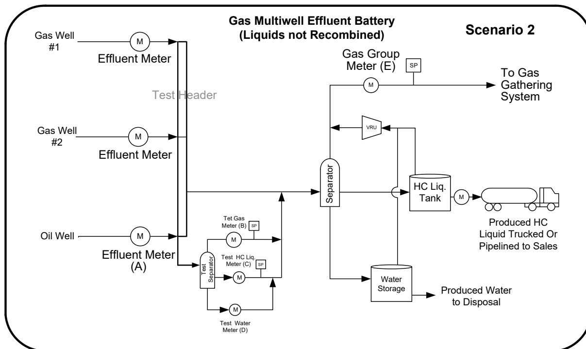
Figure 7.15 Scenario 2 illustration
