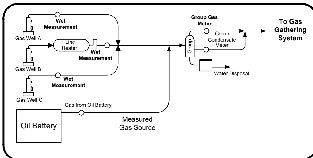
Figure 5.6 Measured oil facility gas delivering into a gas proration battery
