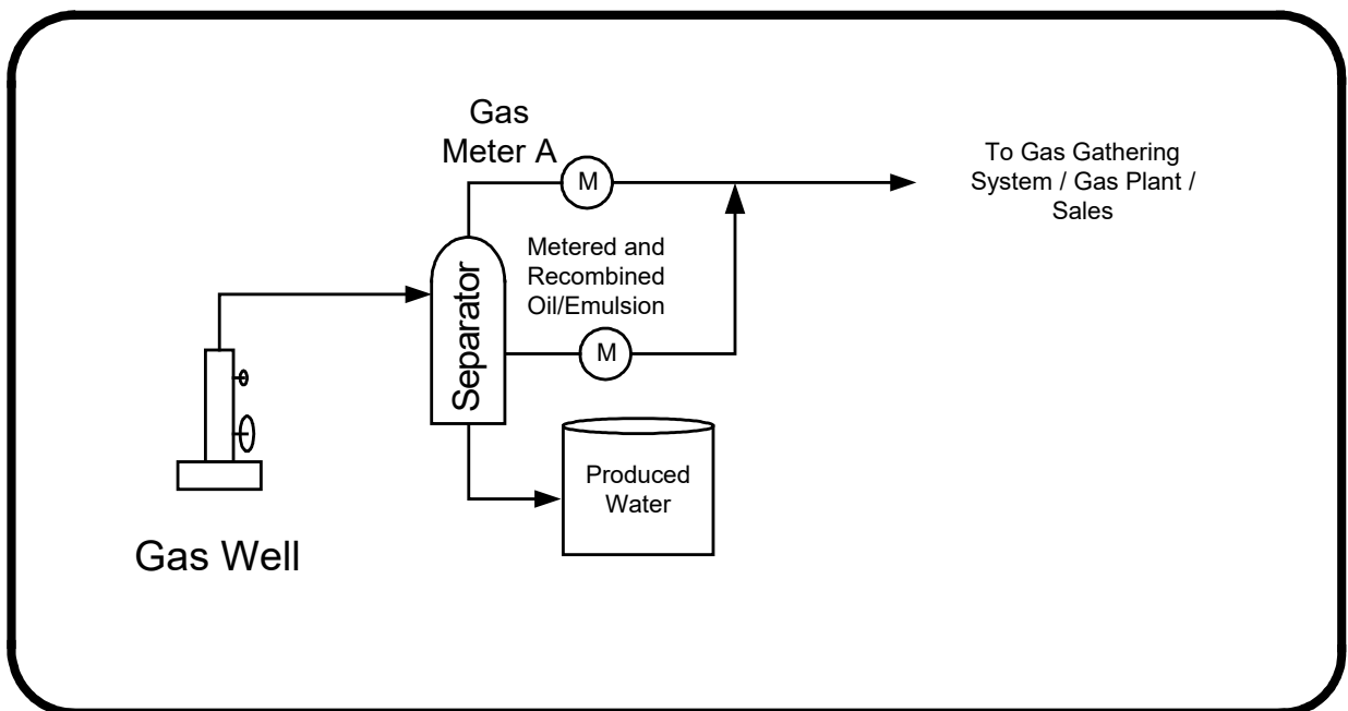
Figure 8.7 Oil production
