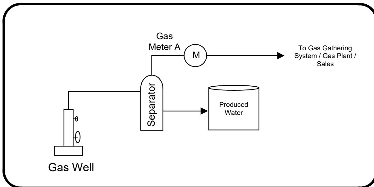
Figure 8.5 Single gas well or multiwell group gas battery and shallow gas well or coalbed methane well with no condensate or oil
