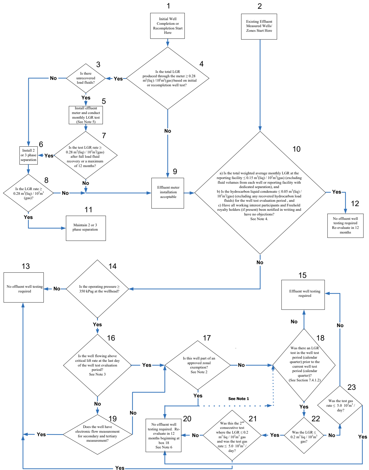
Figure 7.10 Well measurement and testing decision tree. (Text boxes are numbered, left to right.)
