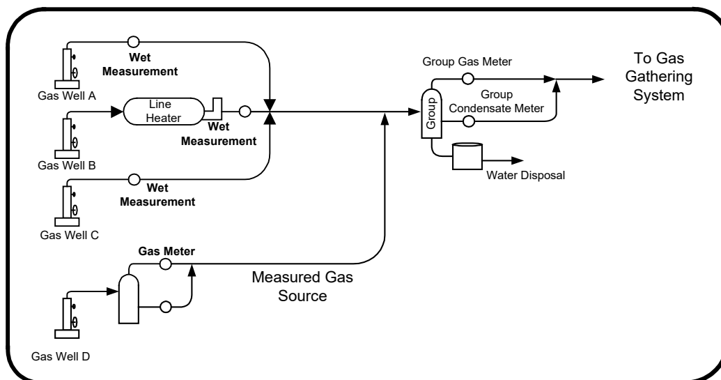
Figure 5.3 Measured gas sources delivering into a gas multiwell effluent measurement battery with battery condensate separated, metered, and recombined with battery gas
