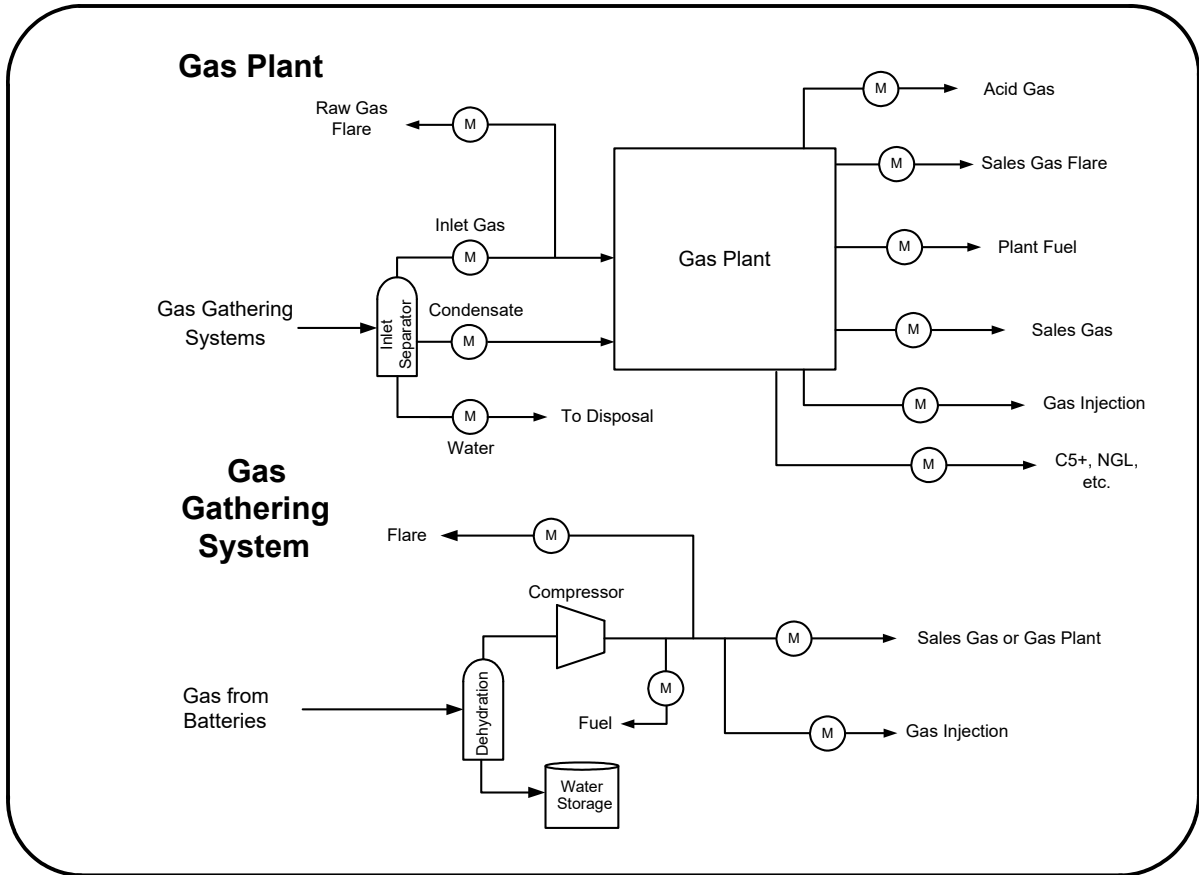
Figure 8.11 Gas plant and gas gathering system
