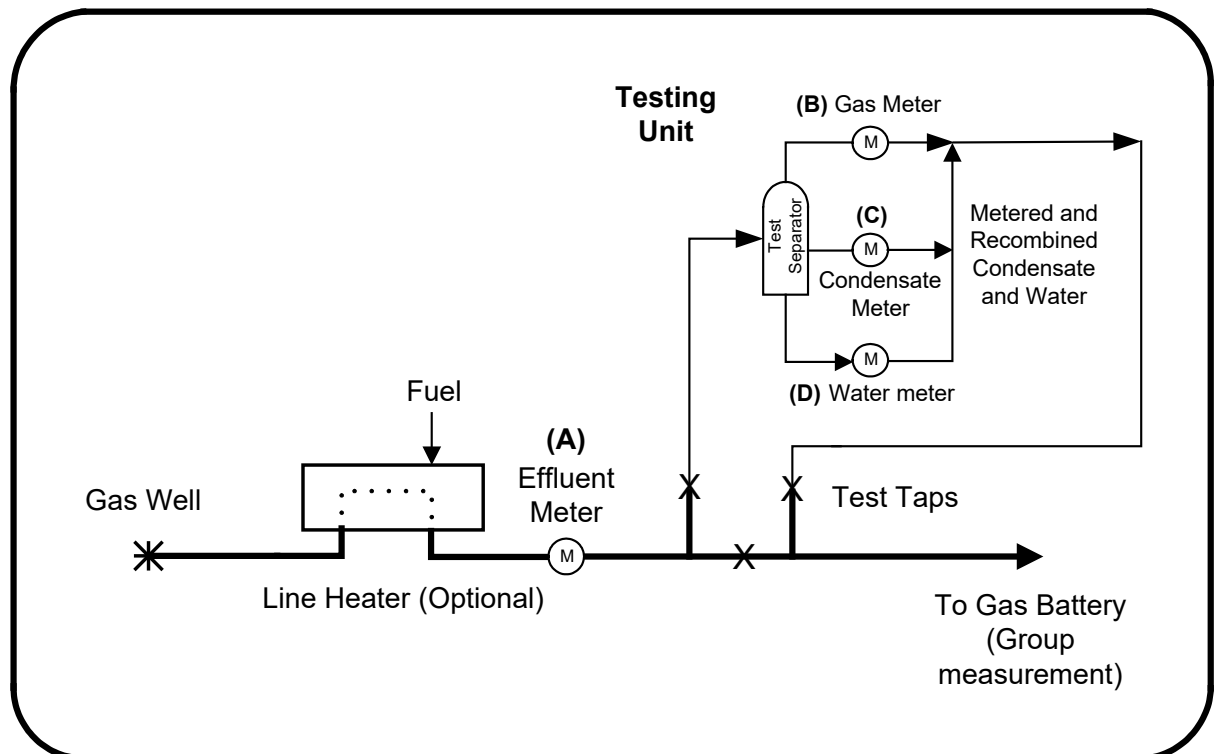
Figure 7.12 Effluent well meter testing configuration with condensate production
