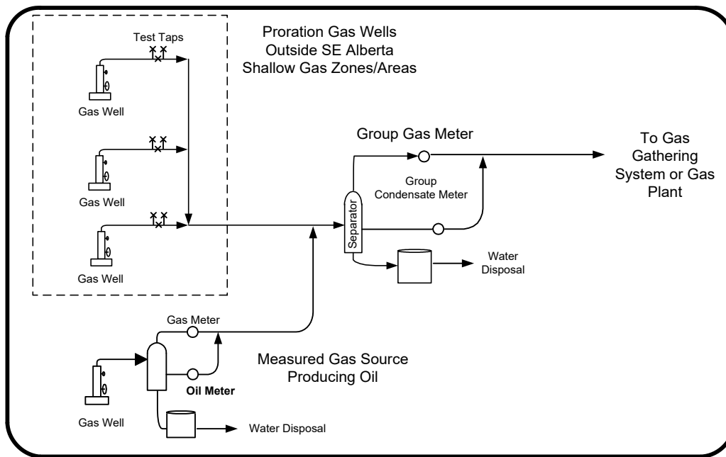
Figure 5.12 Measured oil or oil emulsion from a measured gas source delivering into a gas proration battery or gas plant
