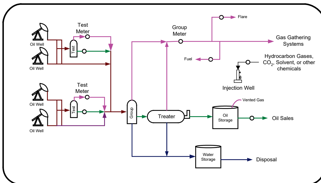
Figure 8.14 Miscible/immiscible flood
