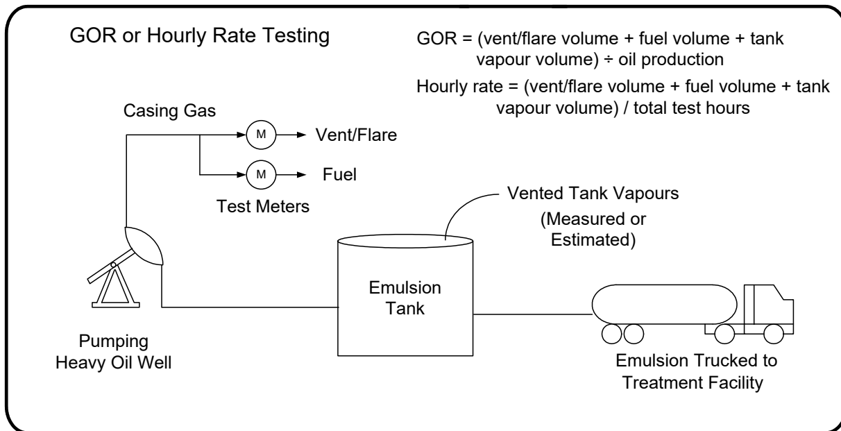
Figure 12.1 GOR or hourly rate testing schematic
