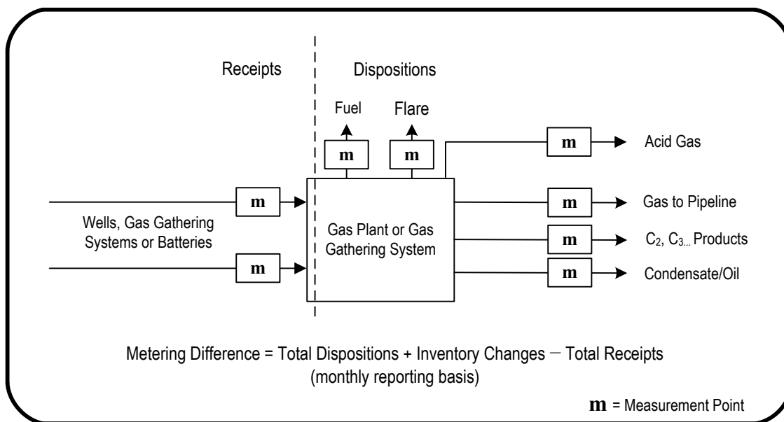
Figure 3.4 Gas plant or gas gathering system
