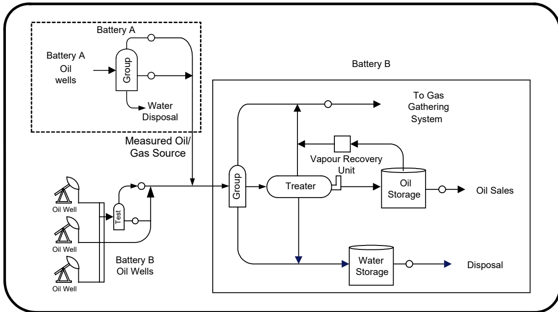
Figure 5.11 Measured oil or oil emulsion (and gas if applicable) under pressure from a battery delivering into a crude oil multiwell proration battery by pipeline
