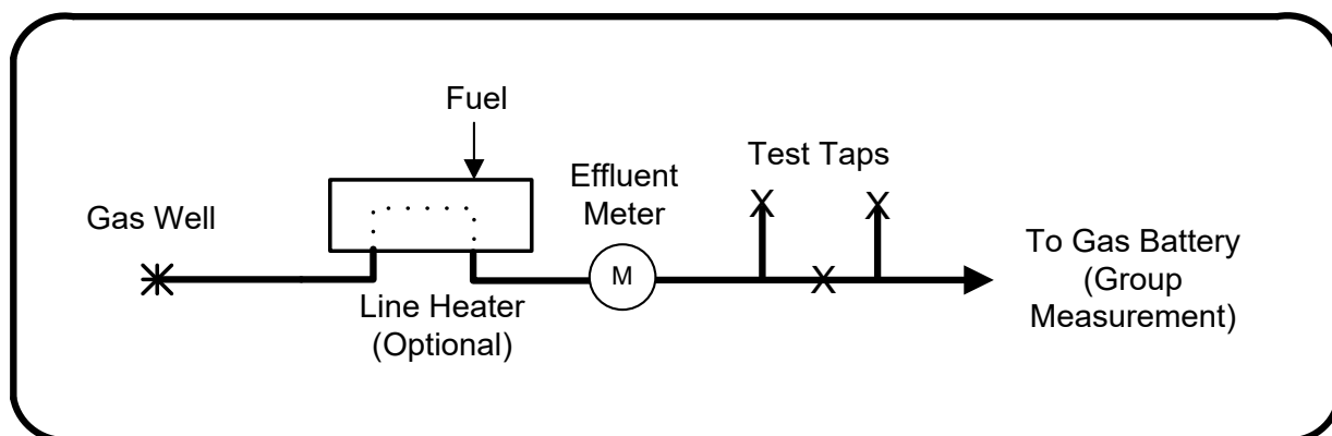
Figure 7.8 Typical gas well effluent metering configuration
