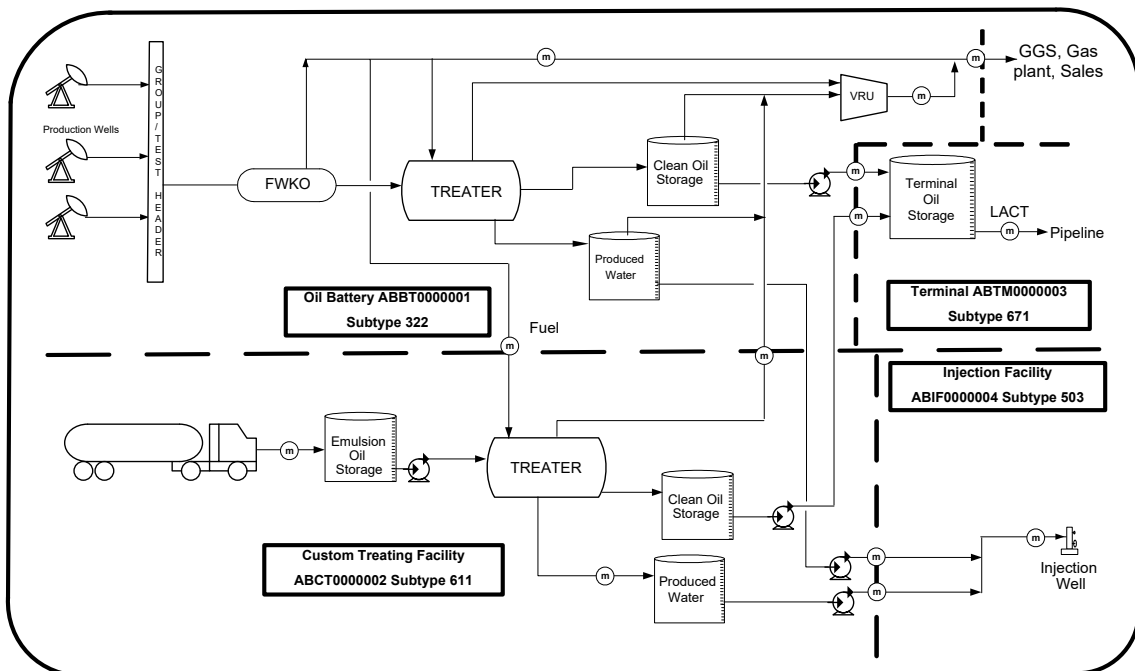
Figure 10.2 Custom treating, oil battery, and terminal schematic – scenario 1
