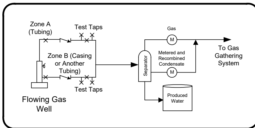
Figure 5.15 Surface comingling of multiple gas zones/wells test method 1
