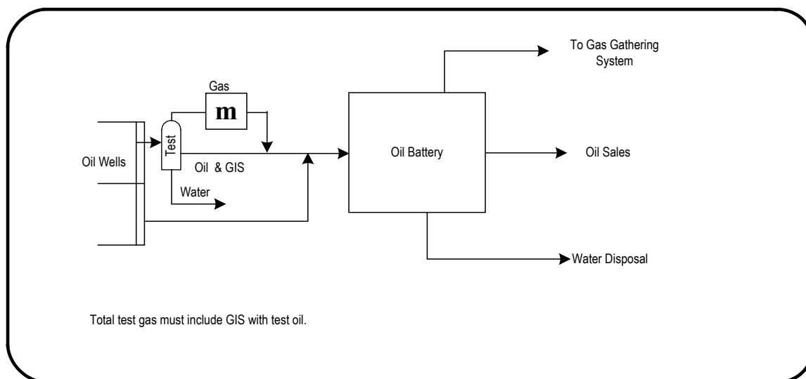
Figure 1.5 Well gas (proration battery)
