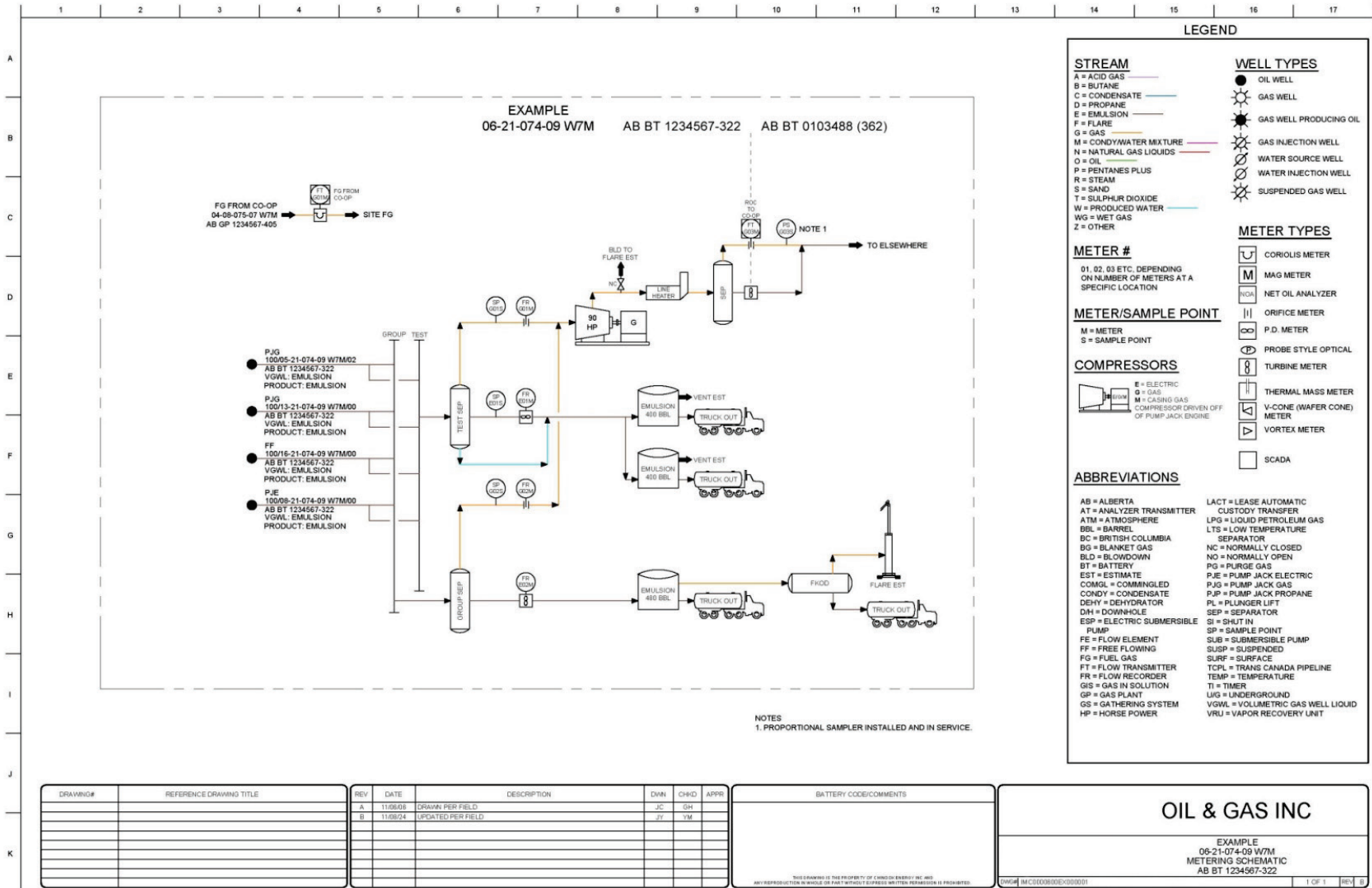
Appendix Figure 5 Sample Schematic Diagram
