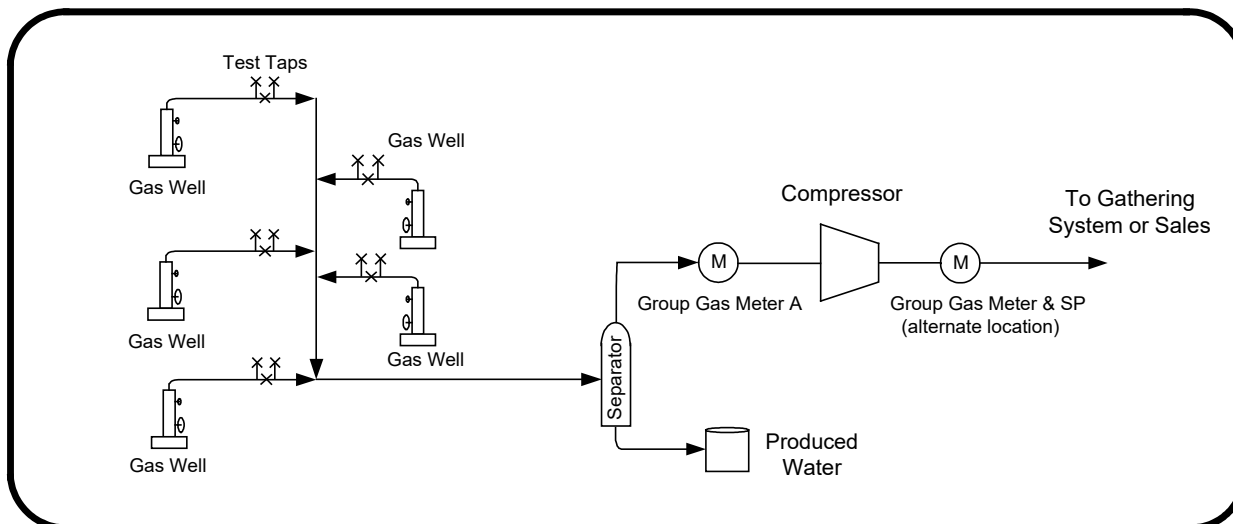
Figure 8.1 Shallow gas or coalbed methane wells
