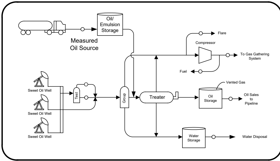
Figure 5.10 Measured oil and/or oil-water emulsion from a battery delivering into a crude oil multiwell proration battery
