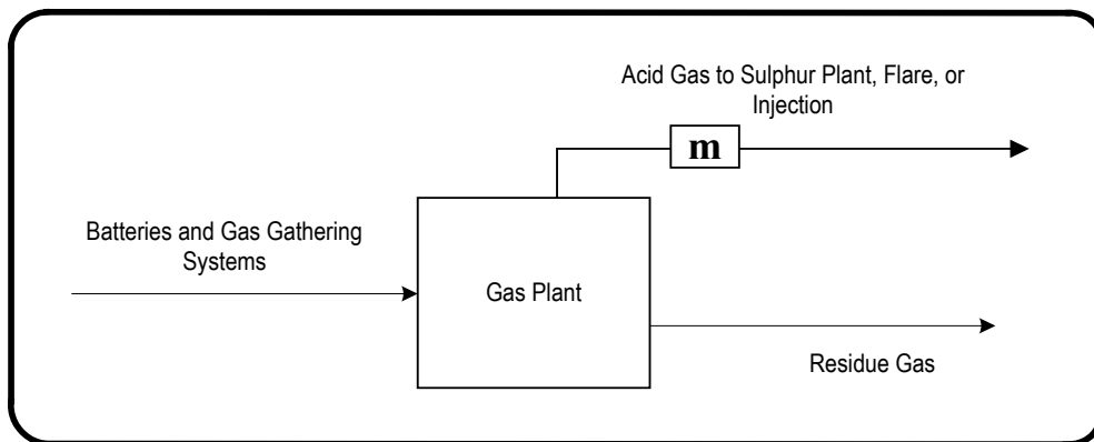
Figure 1.13 Acid gas
