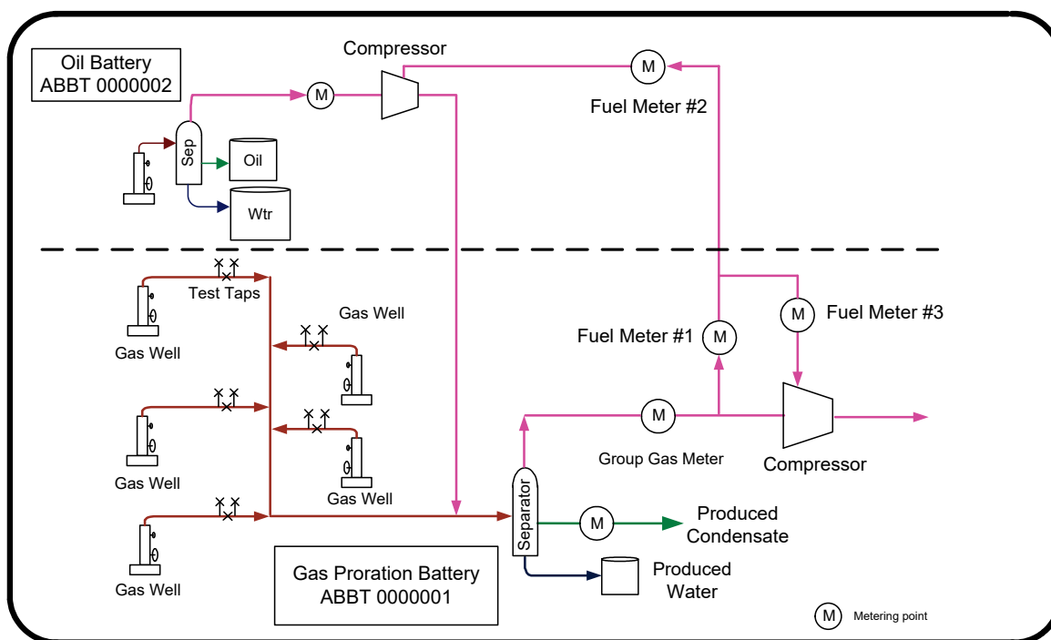
Figure 5.15 Fuel gas measurement by difference scenarios
