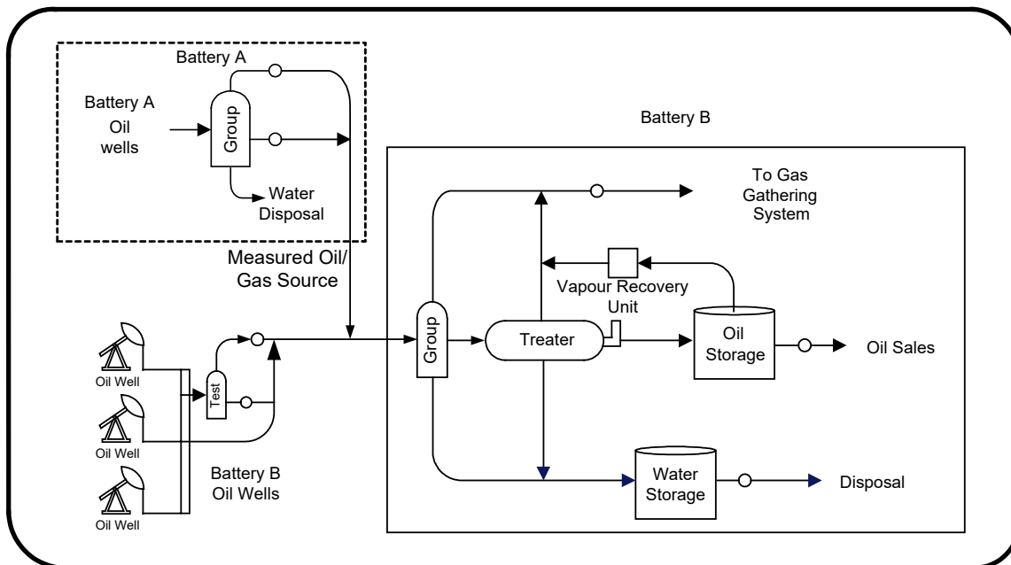
Figure 5.14 Oil battery example of volumetric criteria for measured oil tying into a proration battery
