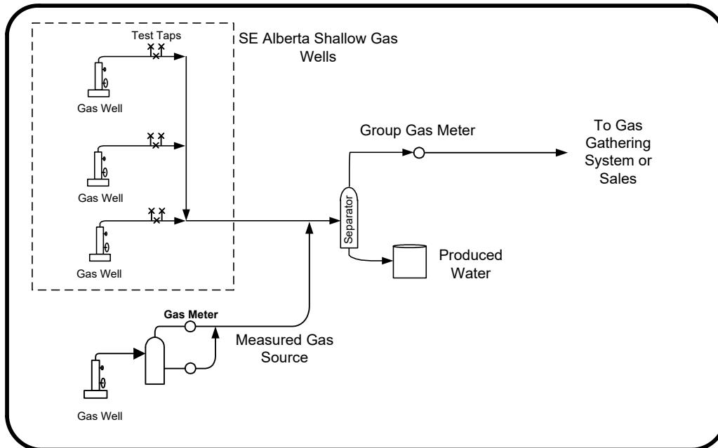
Figure 5.1 Measured gas source delivering into a gas multiwell proration SE Alberta battery
