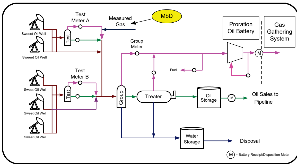
Figure 5.7 Measured gas coming into oil battery with MbD
