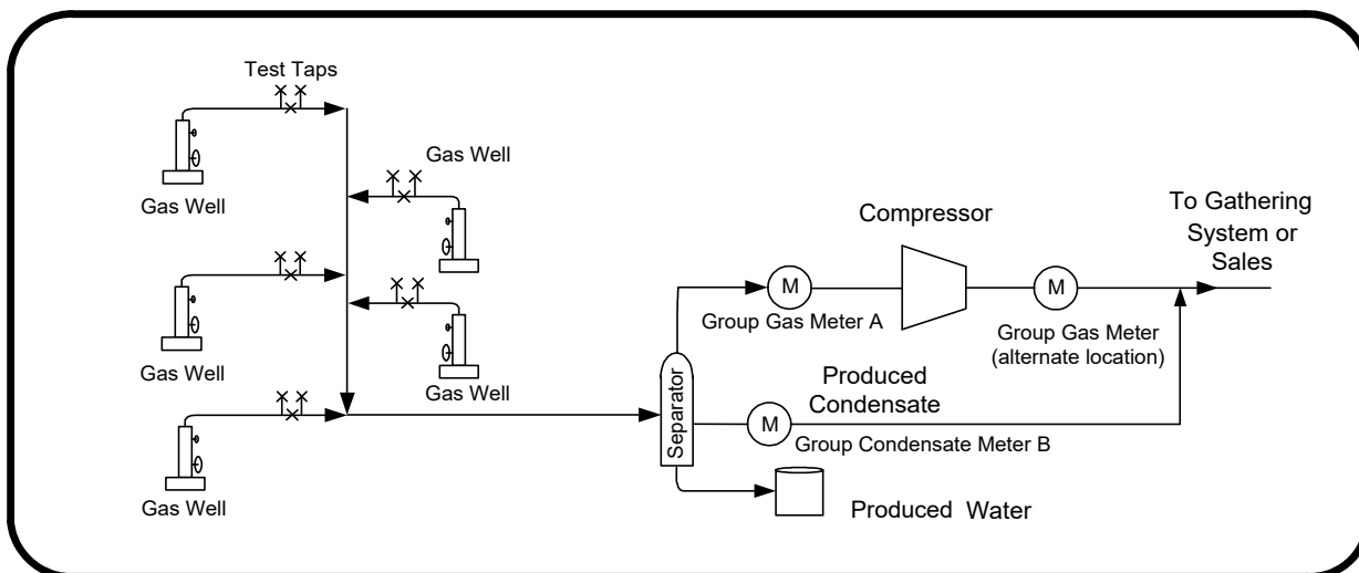
Figure 8.2 Gas multiwell proration outside SE Alberta battery
