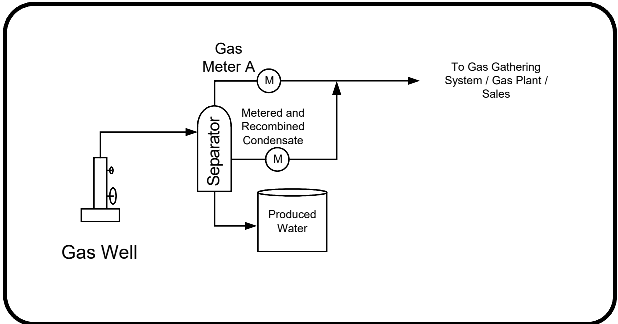
Figure 8.6 Condensate production
