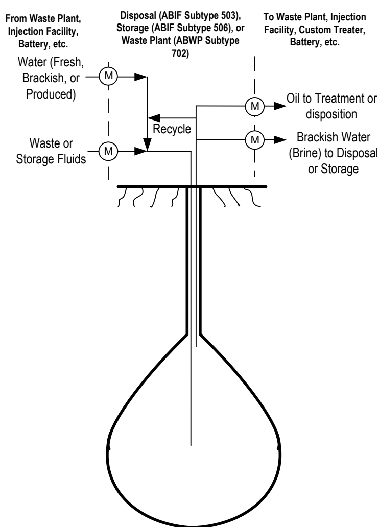
Figure 15.2 Cavern measurement
