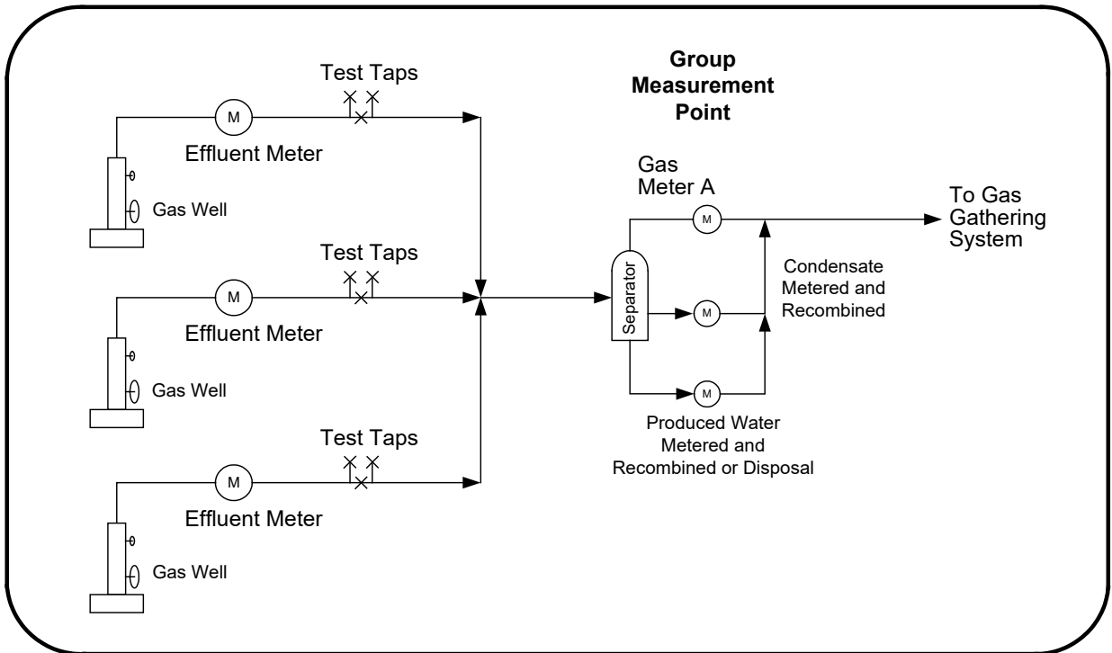
Figure 8.3 Typical multiwell effluent proration battery
