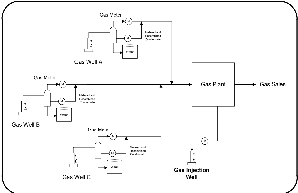
Figure 8.9 Gas cycling scheme
