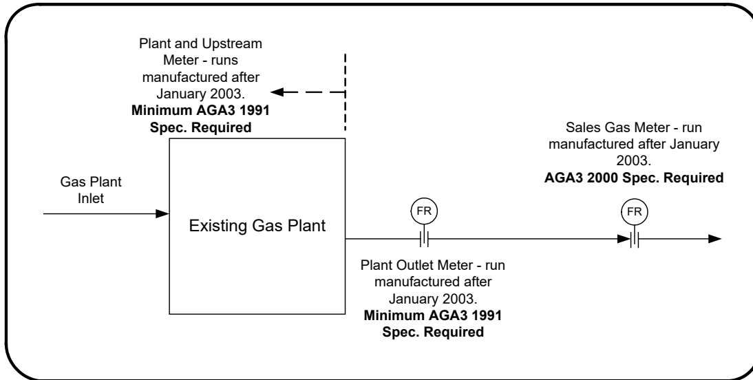
Figure 4.6 Gas plant outlet meter AGA3 1991 specification requirements
