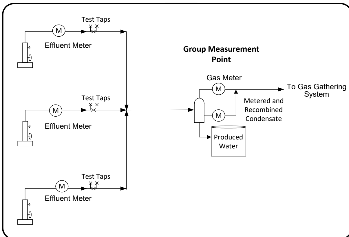
Figure 7.7 Typical gas multiwell effluent measurement proration battery configuration
