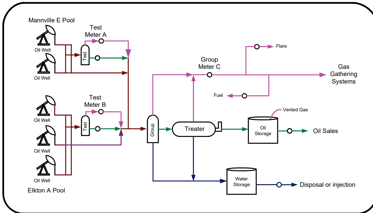
Figure 8.13 Primary production/water flood
