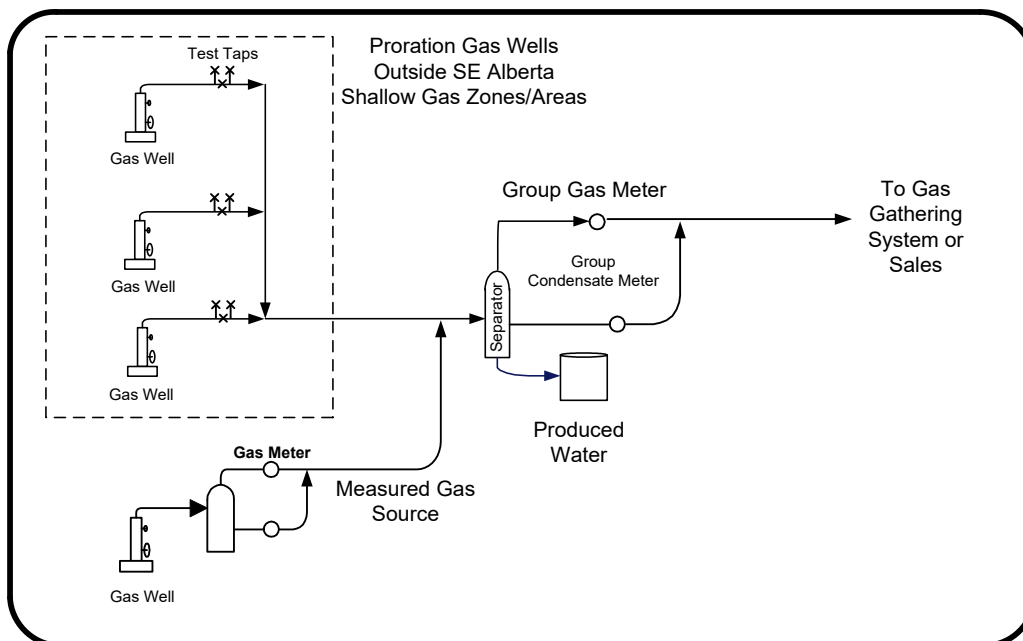
Figure 5.2 Measured gas source delivering into a gas multiwell proration outside SE Alberta battery
