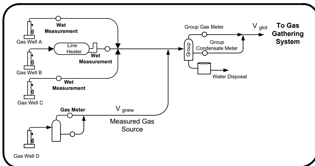
Figure 5.13 Gas battery example of volumetric criteria for measured gas tying into a proration battery
