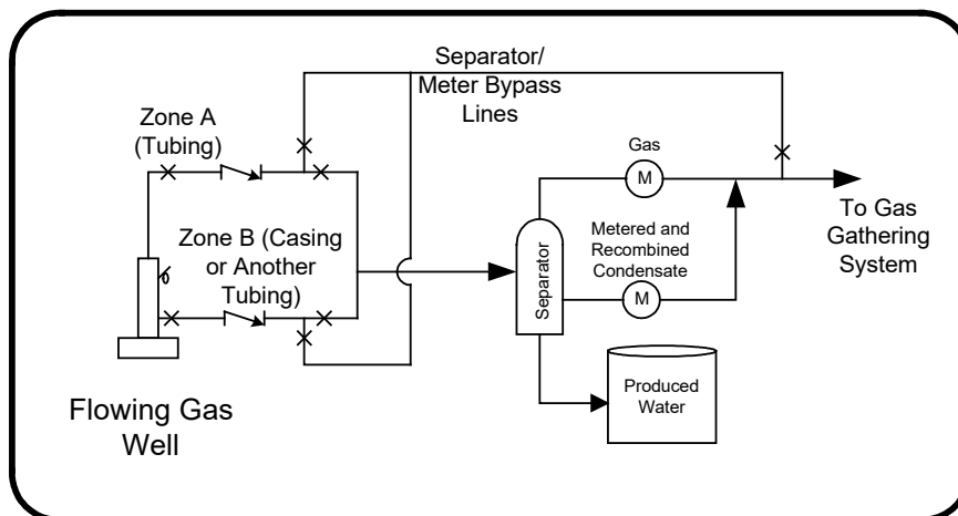
Figure 5.16 Surface comingling of multiple gas zones/wells test method 2
