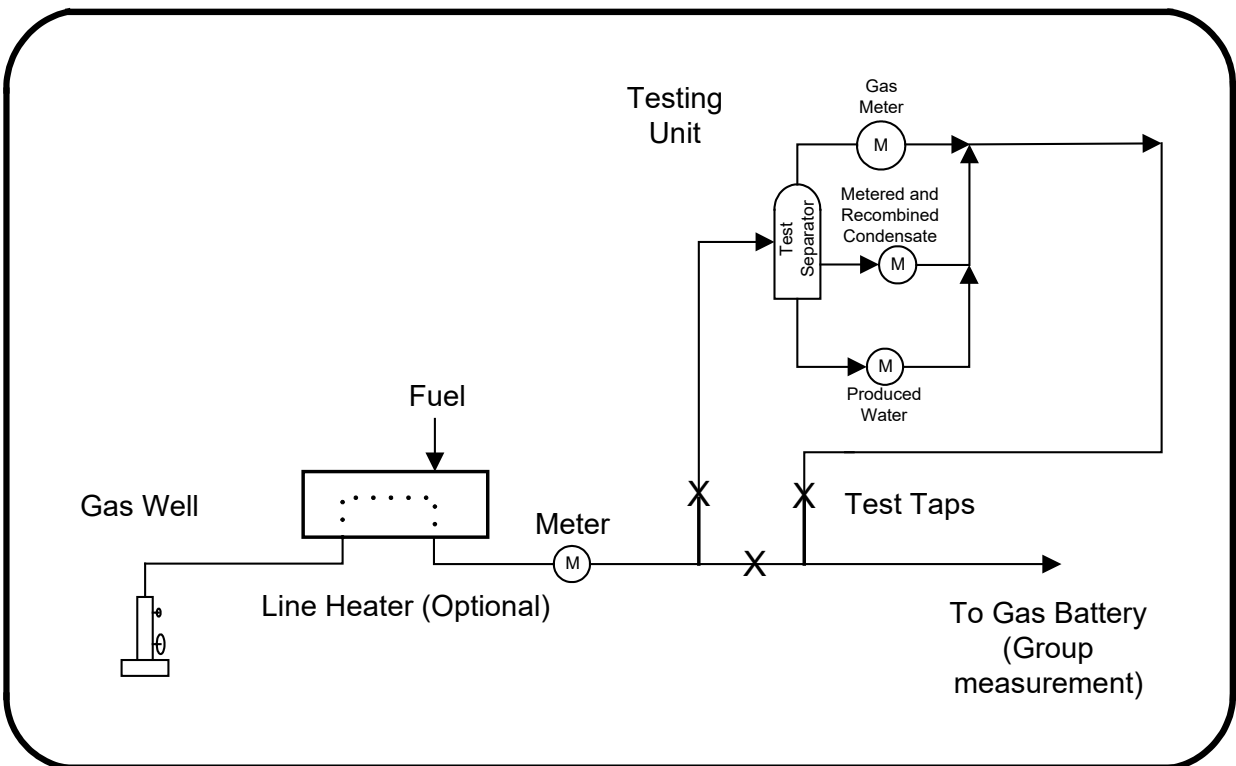
Figure 8.4 Typical effluent well testing configuration
