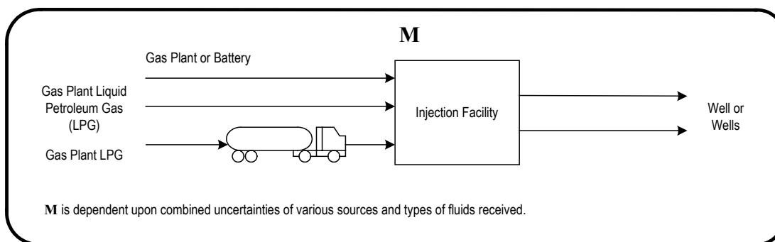
Figure 1.21 Total gas
