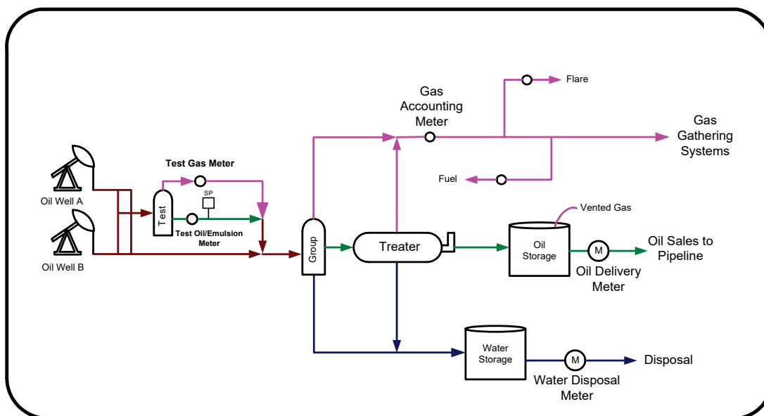
Figure 6.3 Proration testing battery
