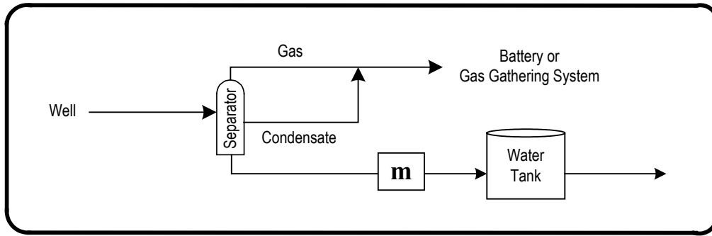
Figure 1.20 Well water
