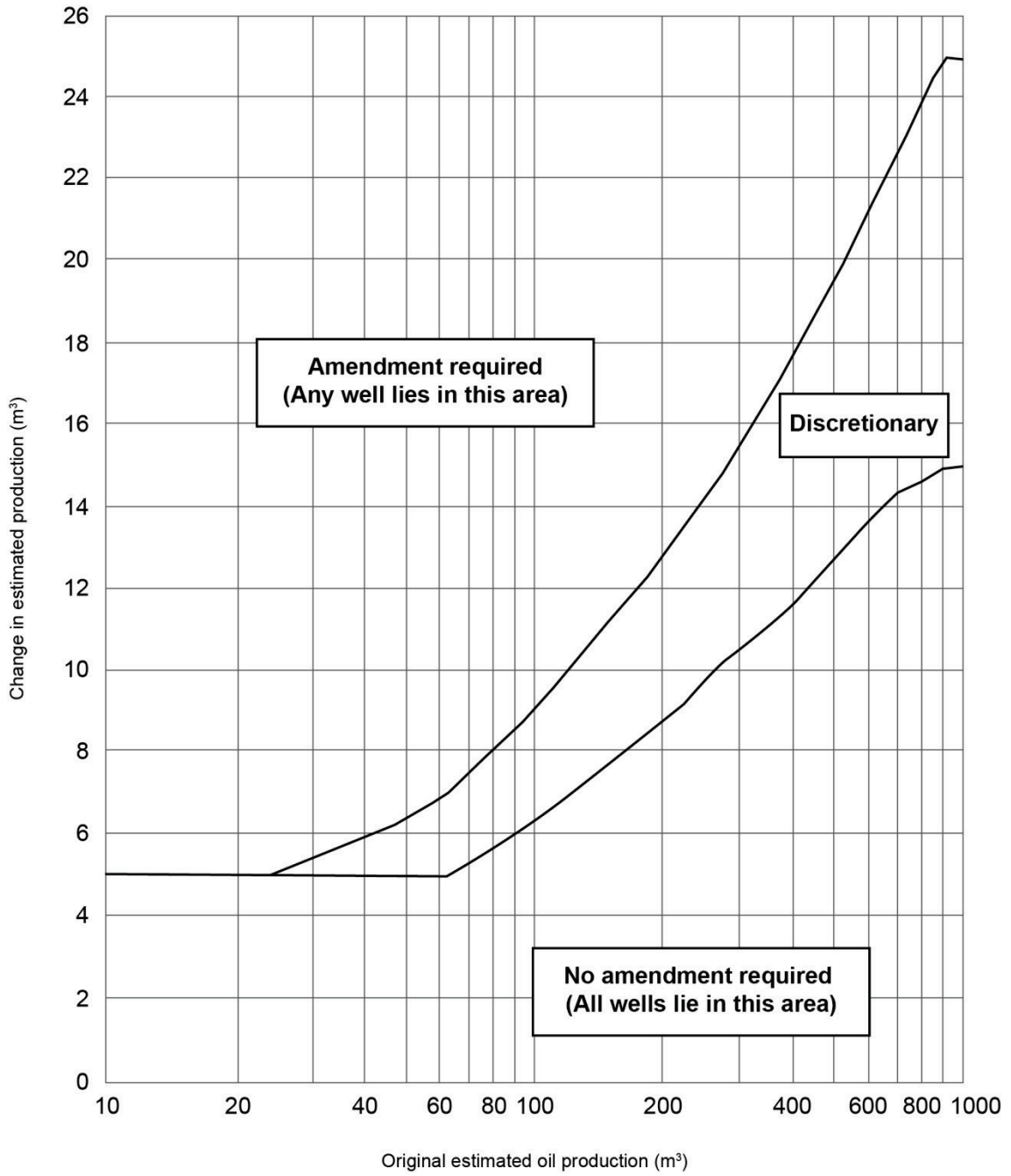
Figure 6.2 Criteria for determining when volumetric amendments are required on a per well basis
