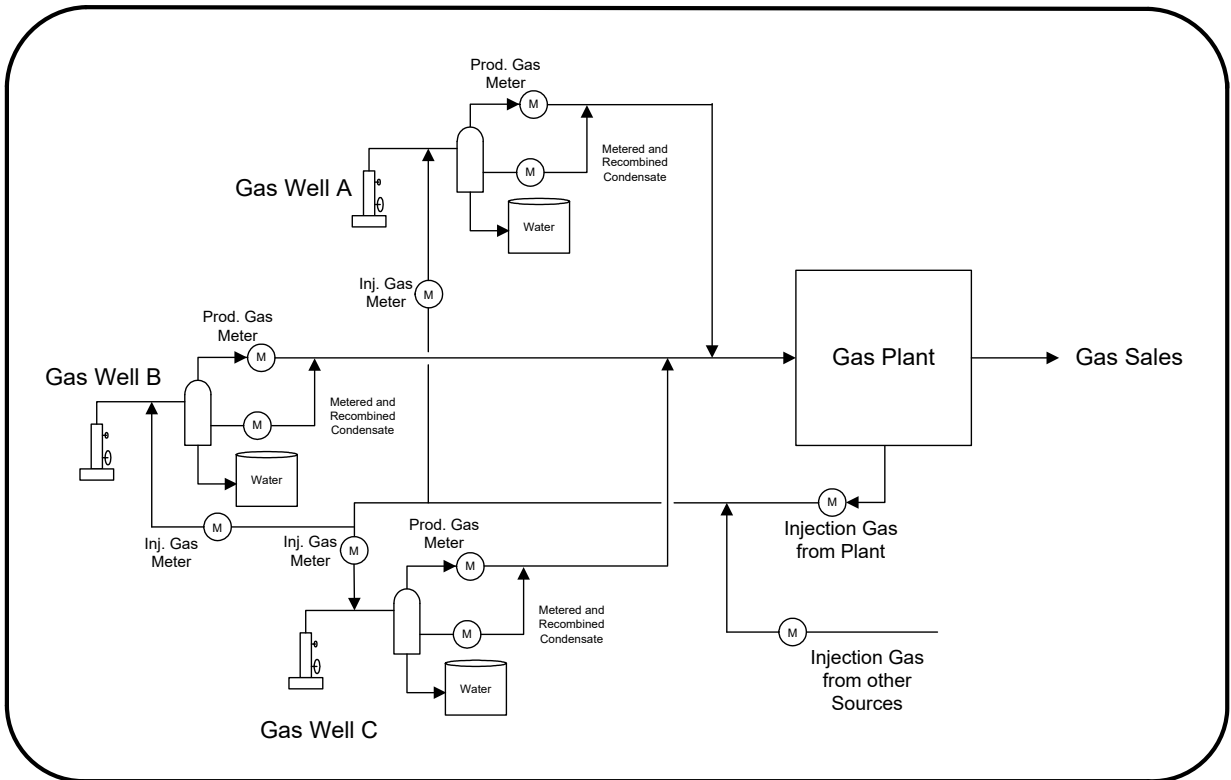
Figure 8.8 Gas storage scheme
