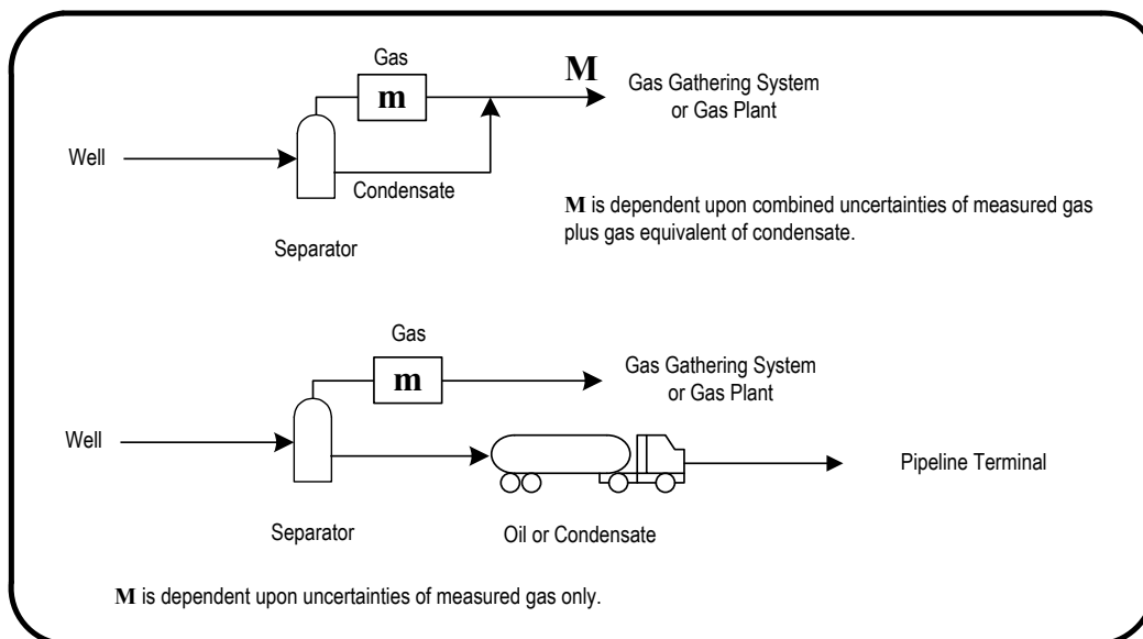
Figure 1.15 Well gas (well site separation)
