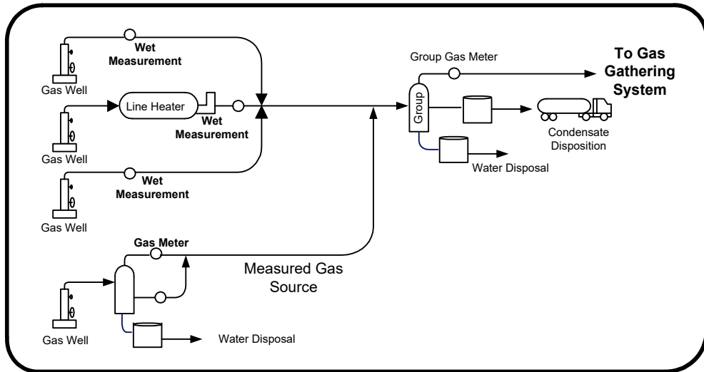
Figure 5.4 Measured gas sources delivering into a gas multiwell effluent measurement battery with battery condensate separated and sent to a tank for disposition to sales
