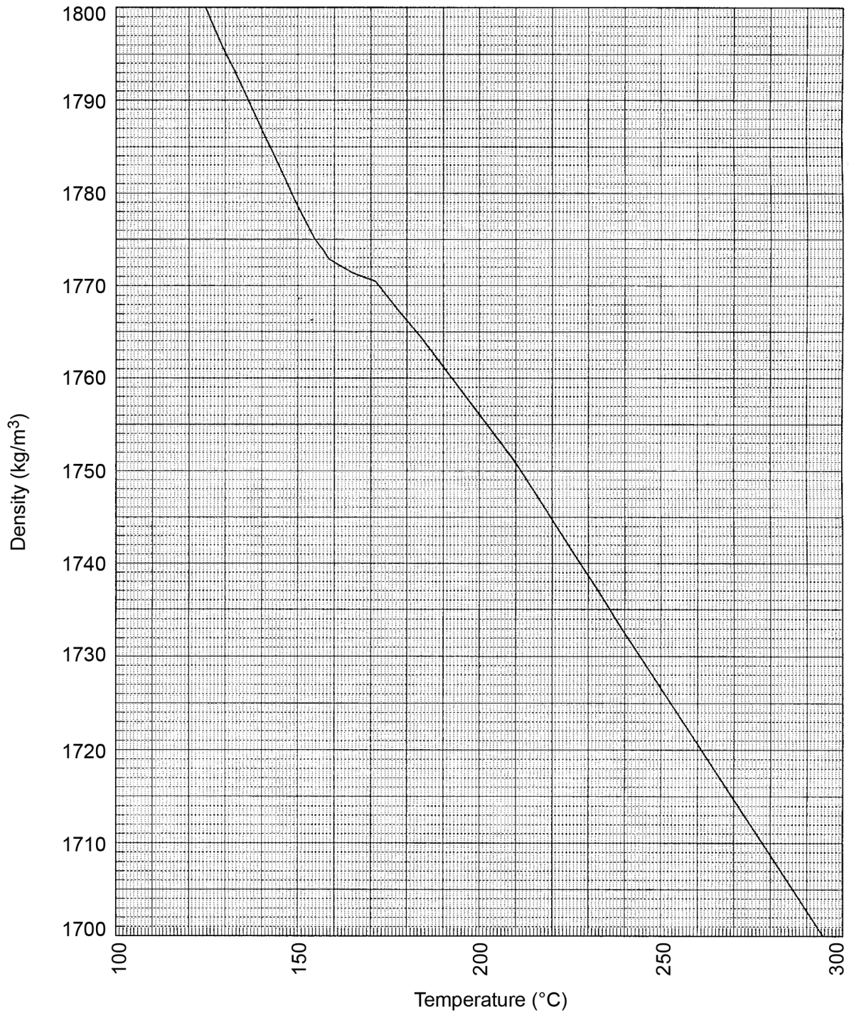
Figure 11.1 Liquid sulphur density vs. temperature
