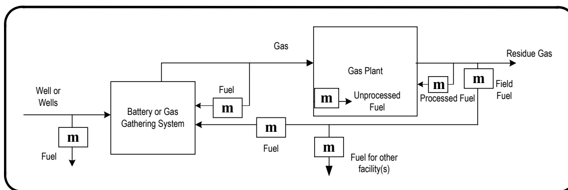
Figure 1.11 Fuel gas
