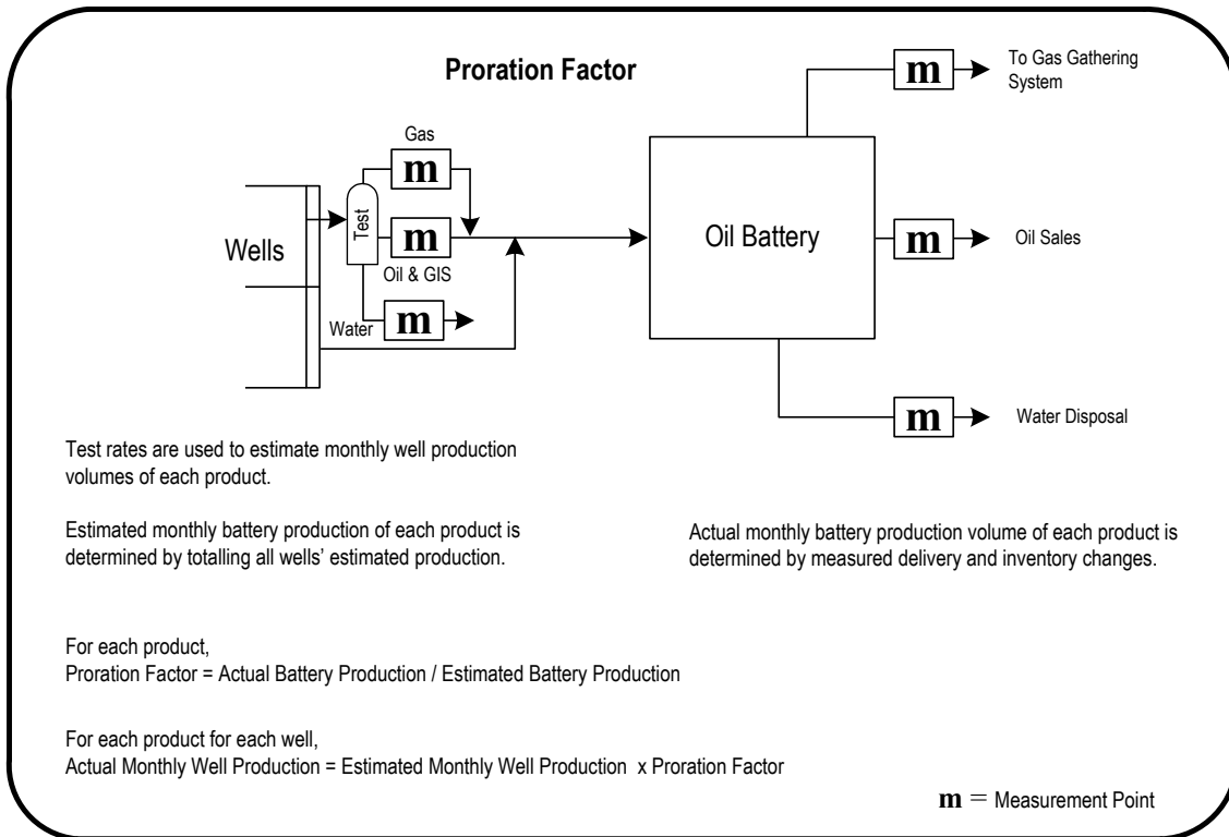
Figure 3.1 Proration factor
