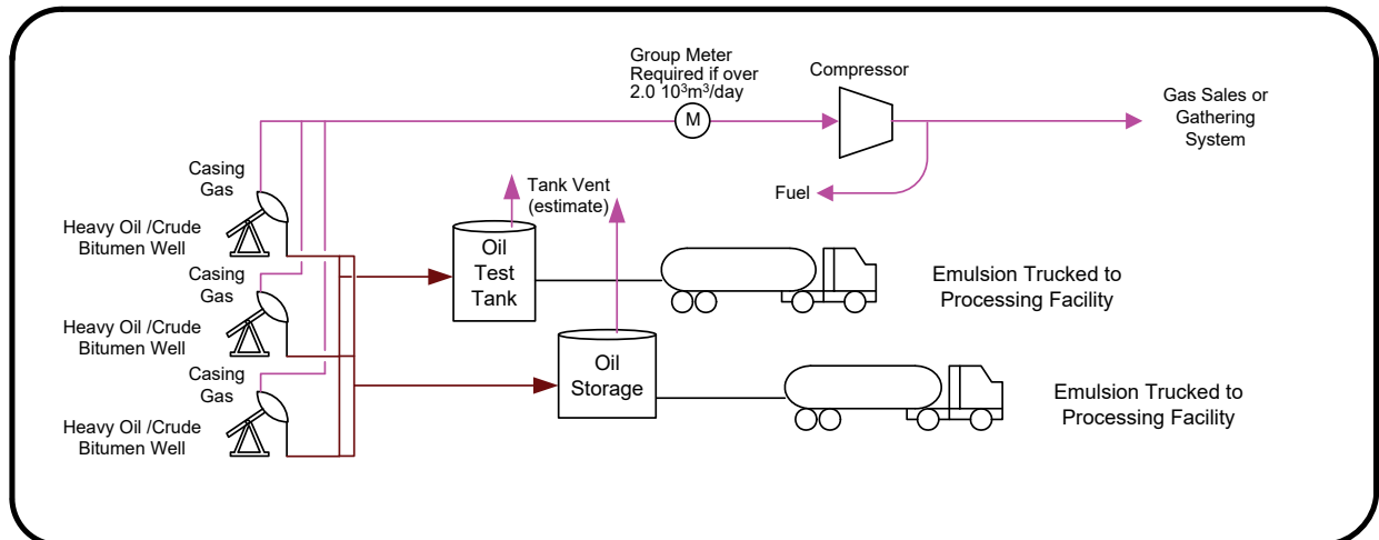
Figure 8.17 Heavy oil / crude bitumen multiwell proration battery
