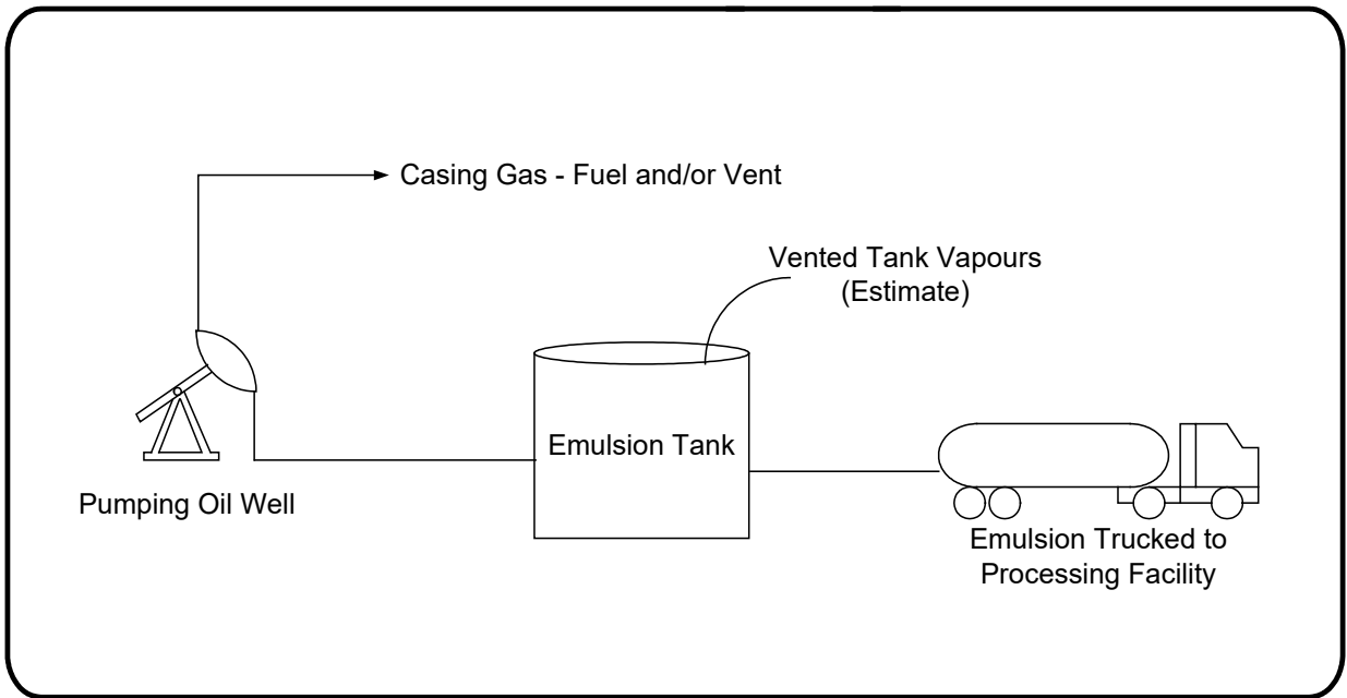
Figure 8.15 Heavy oil/crude bitumen single-well battery
