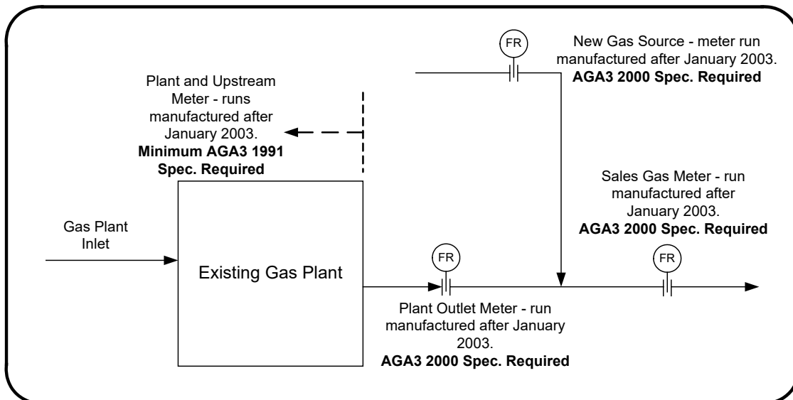
Figure 4.7 Gas plant outlet meter AGA3 2000 specification requirements
