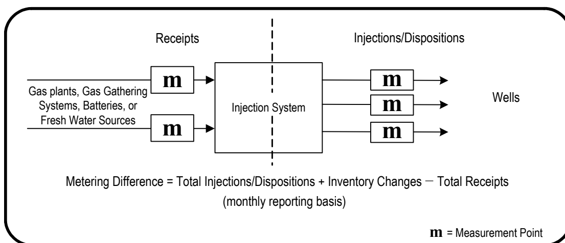
Figure 3.3 Injection/disposal systems
