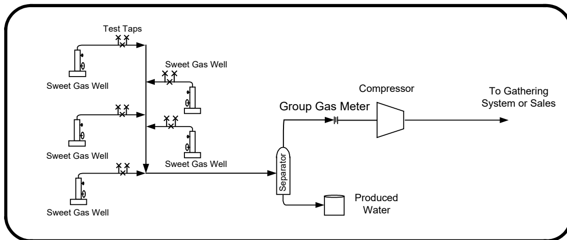
Figure 7.1 Typical SE Alberta shallow gas battery
