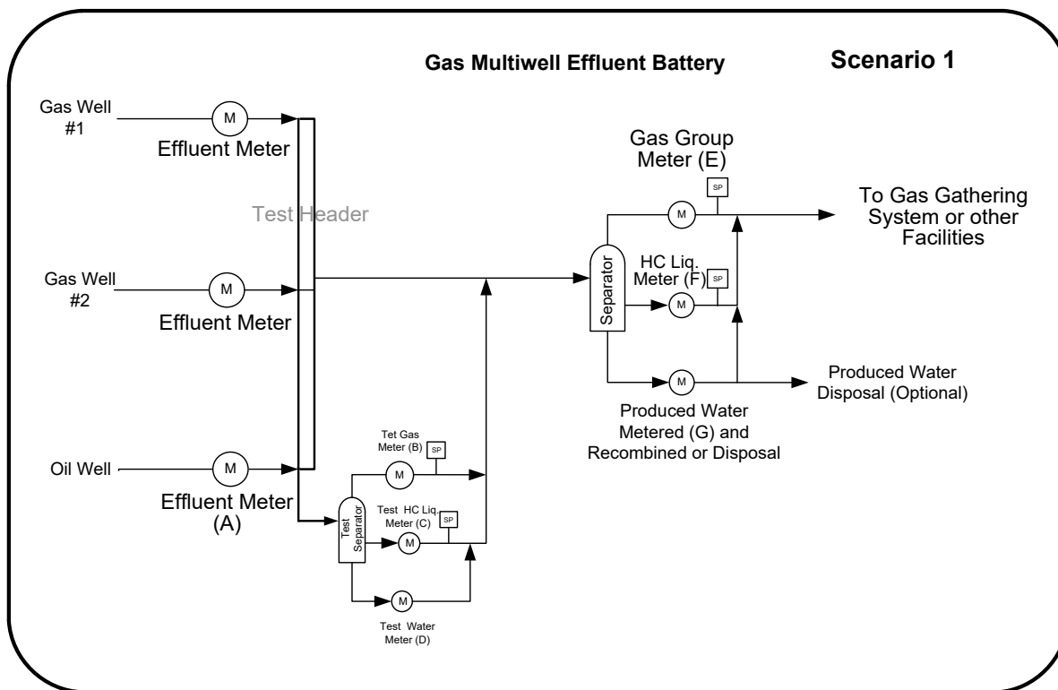
Figure 7.14 Scenario 1 illustration
