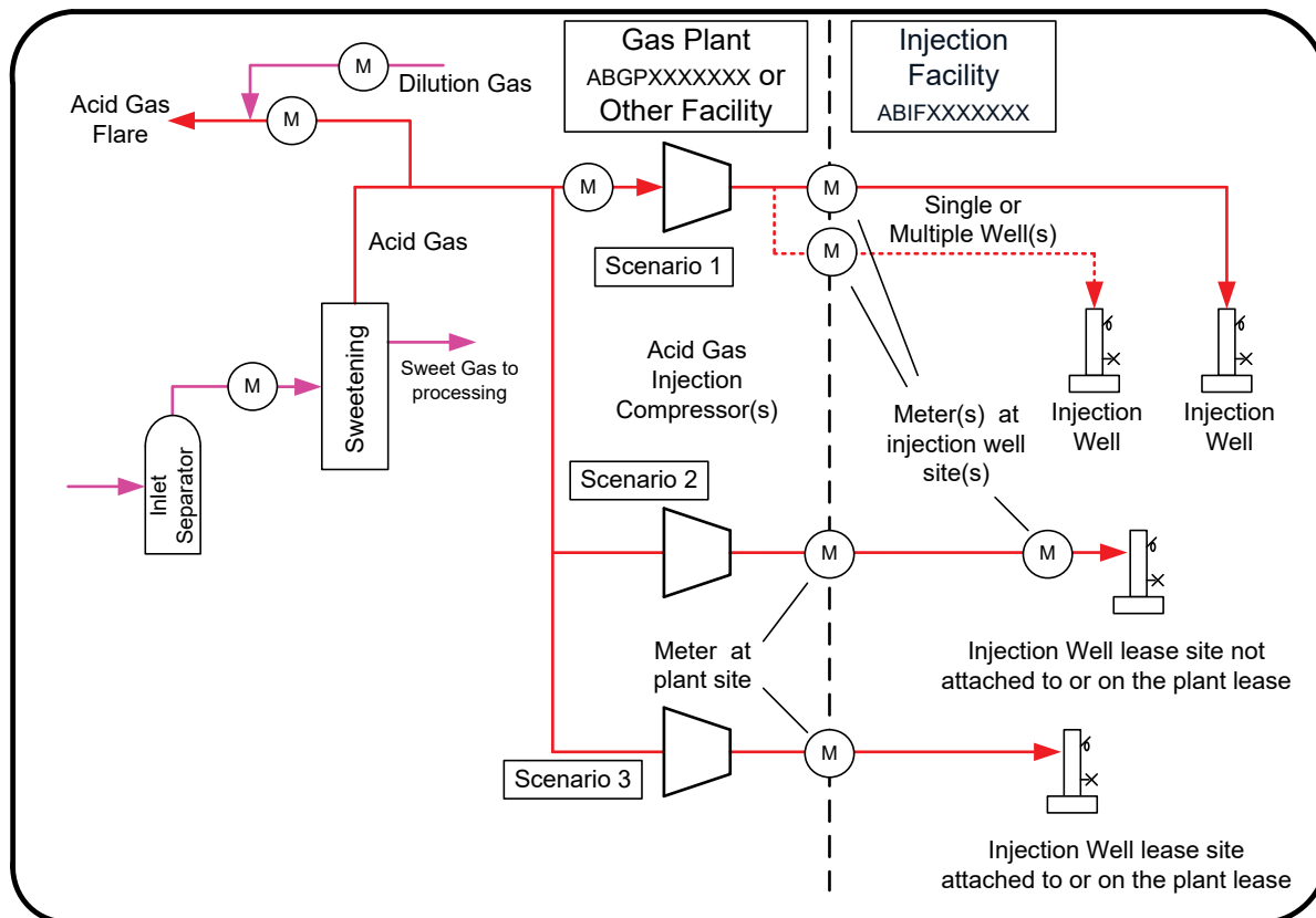
Figure 11.3 Acid gas injection measurement scenarios
