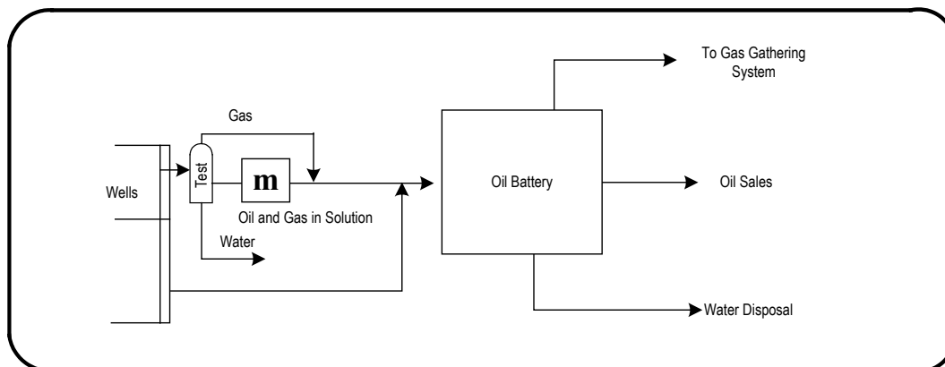
Figure 1.4 Well oil (proration battery)
