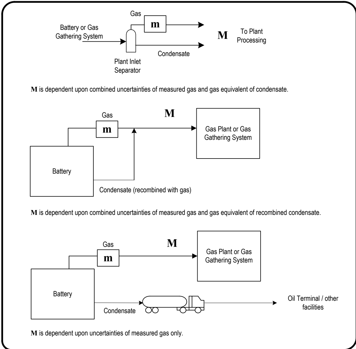
Figure 1.9 Plant inlet or total battery/group gas
