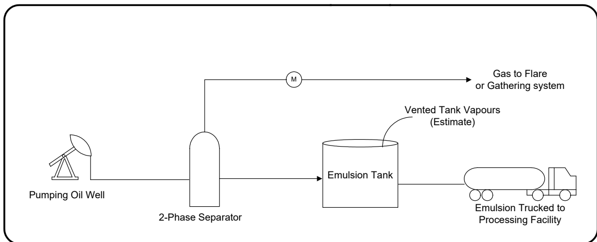
Figure 8.12 Single-well or multiwell group oil battery
