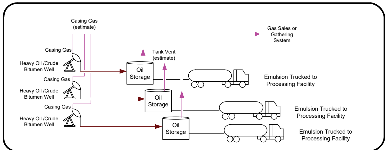
Figure 8.16 Heavy oil/crude bitumen multiwell group battery
