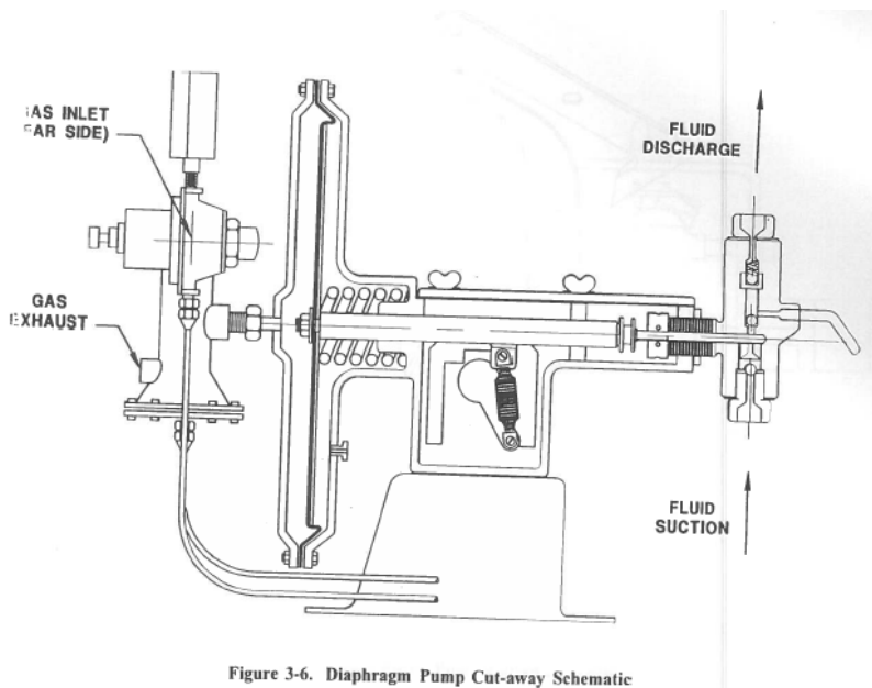
Figure 3-6. Diaphragm Pump Cut-away Schematic
