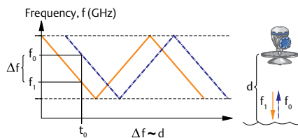
Figure 2.12: The FMCW method.
