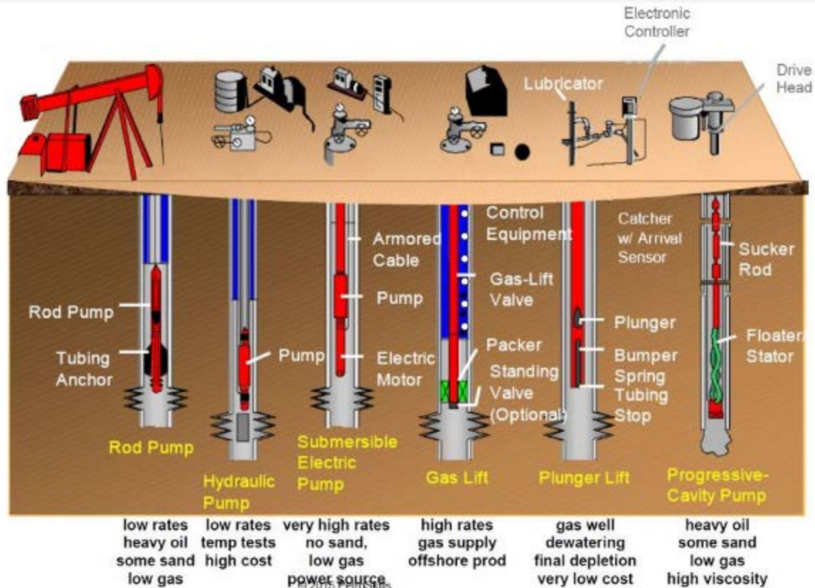
Figure 1-1 Examples of the primary methods of artificial lift.
