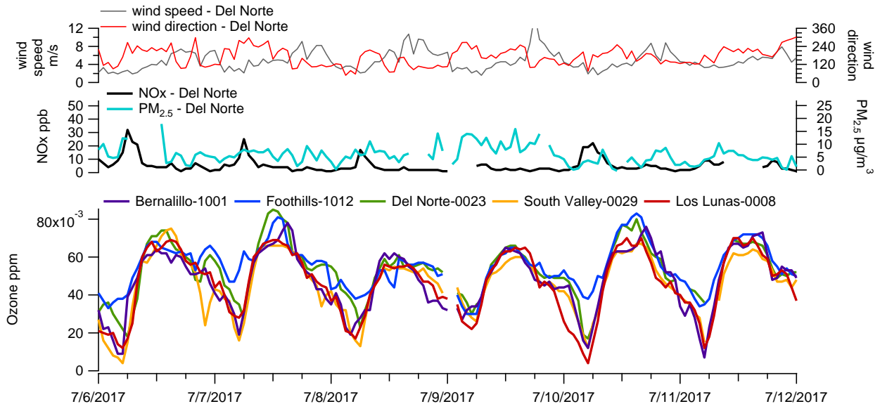
Figure 23. Time series of ozone in the Albuquerque MSA, and NO x , PM 2.5 , wind speed, and wind direction at the Del Norte site during July 6-12, 2017.
