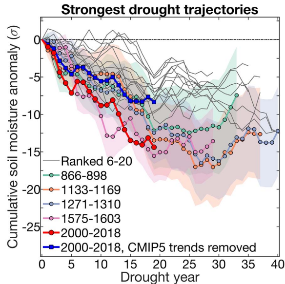
Fig. 3. Development of the most severe 19-year droughts since 800 CE. Time series of cumulative SWNA summer soil-moisture anomalies for the 20 prolonged droughts with the most-negative 19-year soil-moisture anomalies. The drought periods analyzed here begin 18 years before the most-negative 19-year anomaly. The dark blue line shows 2000–2018 cumulative anomalies after removing CMIP5 multimodel mean climate trends. The shaded regions represent 95% confidence intervals for the four reconstructed megadroughts shown with the light colored lines.
