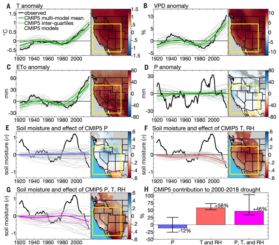
Fig. 2. Effects of anthropogenic climate trends.
